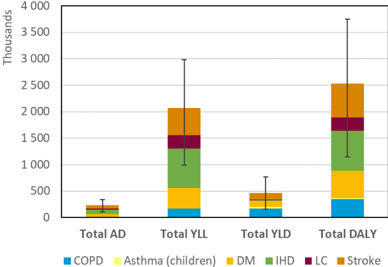
Figure 4.10: Burden of disease indicators for PM2.5 (all countries) differentiated by outcomes. The total is estimated based on the average CRF (bars) and the lower and upper 95% CI (error bars)
